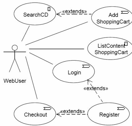
(a) Use case model
