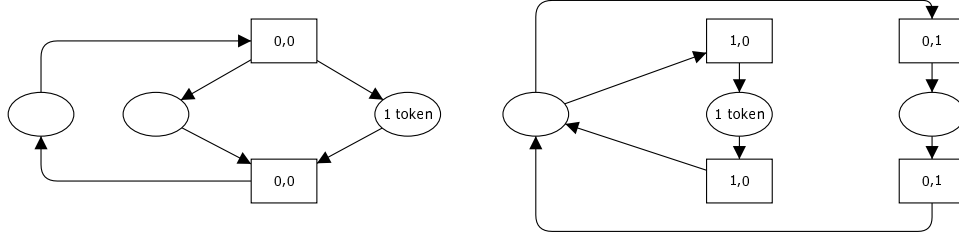
Figure 9. Low-system BPS^{low} (left) and high-system BPS^{high} (right) of the BP-system from Fig. 7
