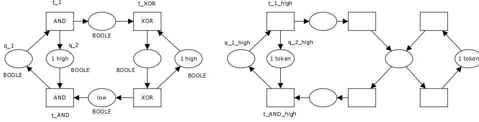
Figure 17. Deadlocking circle (left) and high-system (right)
