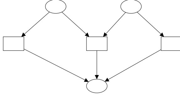
Figure 2. Type of structural conflict which is forbidden for free-choice nets
