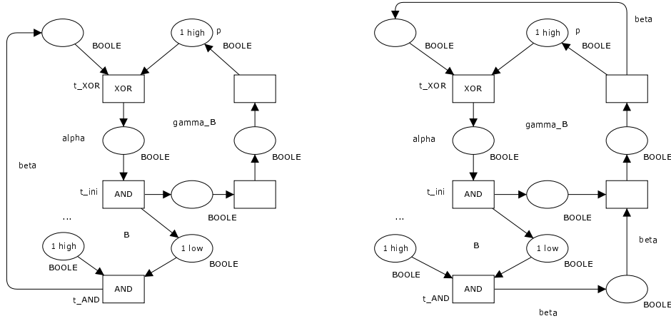
Figure 18. Two BP-systems with a deadlocking circle of size m = 1
