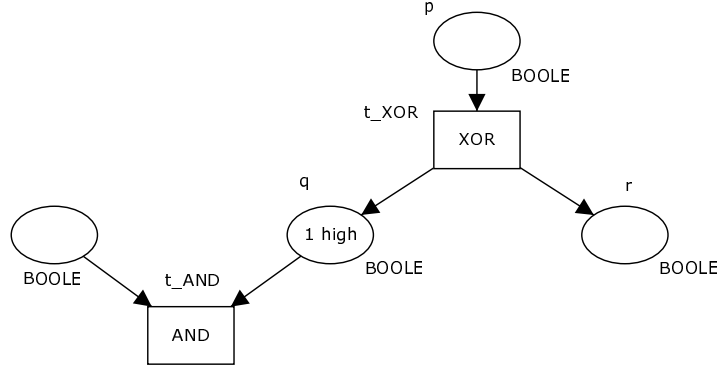
Figure 20. Closing AND-transition t_{AND} \in post(s) in case s = q
