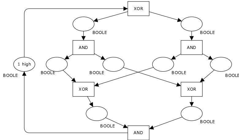
Figure 10. Safe and high-live BP-system BPS_1
