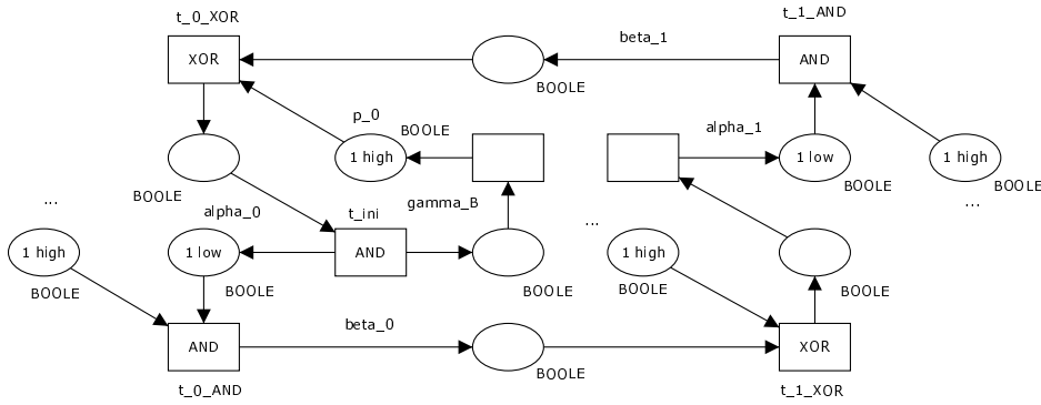
Figure 19. Deadlocking circle of size m = 2
