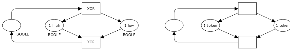
Figure 7. BP-system BPS (left) and its skeleton BPS^{skel} (right)
