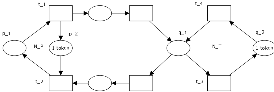
Figure 3. Free-choice system with a frozen token
