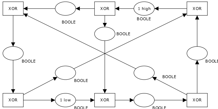
Figure 21. High-live BP-system with enabled T-component and a low-token
