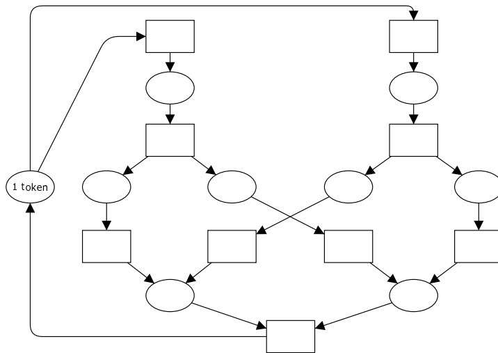
Figure 11. Safe and live high-system BPS_1^{high}
