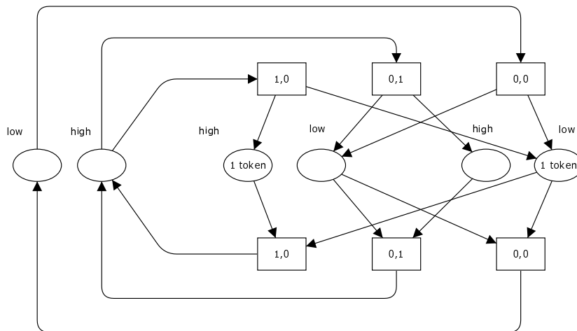
Figure 8. Flattening BPS^{flat} of the BP-system from Fig. 7 (left)
