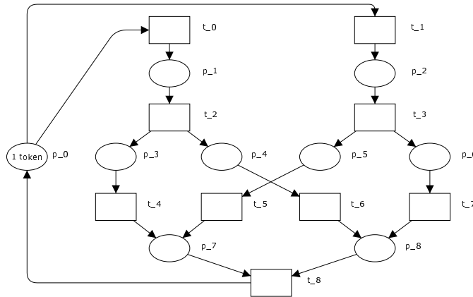
Figure 1. Live and safe restricted free-choice system
