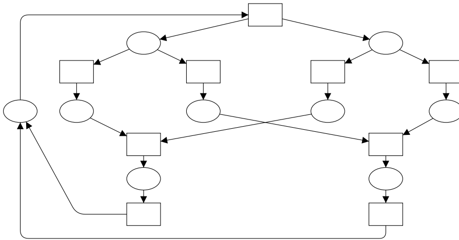
Figure 4. Restricted free-choice net, which is not well-formed
