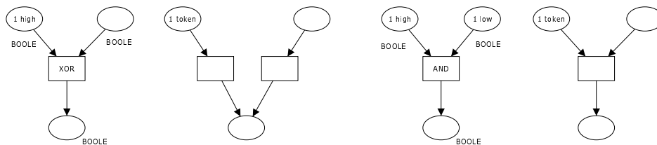
Figure 16. Closing transitions from a dead BP-system and corresponding high-system
