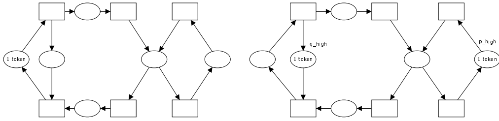
Figure 15. High-system BPS_3^{high} (left) and marking \mu_3^{high} with a frozen token at place q^{high} (right)
