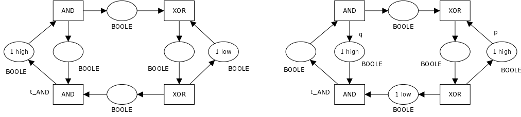
Figure 14. BP-system BPS_3 (left) with a reachable synchronization-deadlock \mu_{3,dead} (right)
